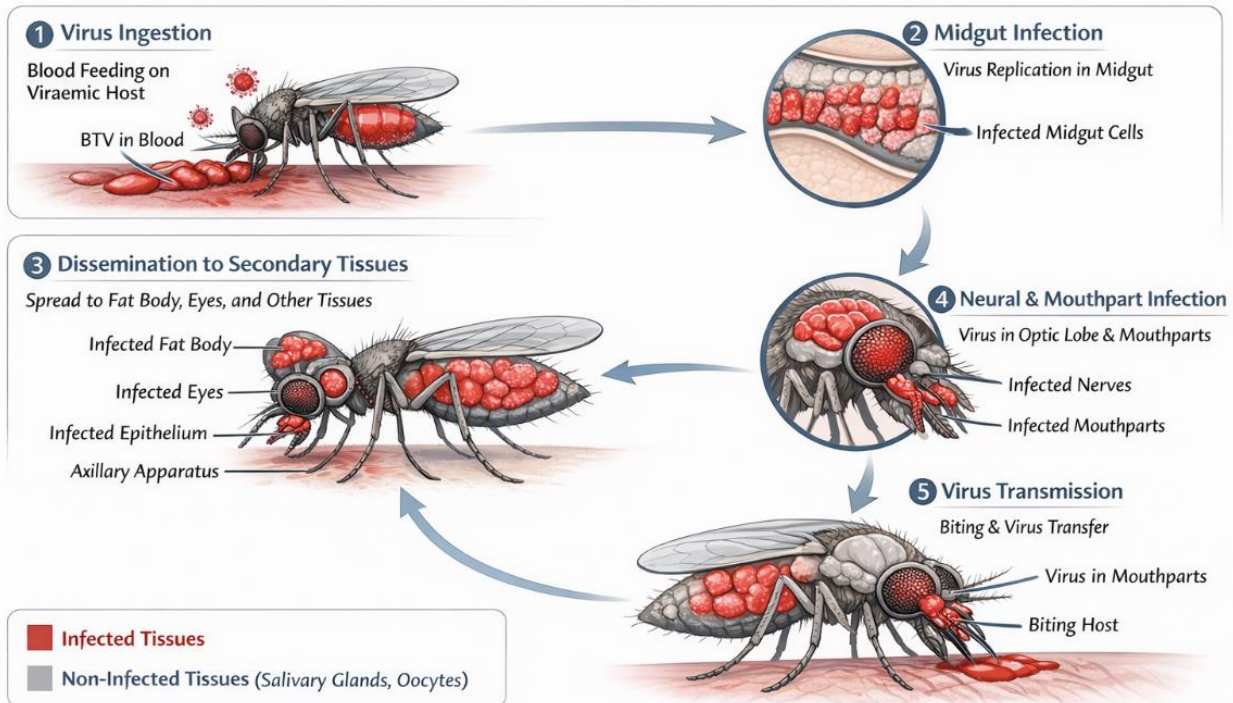
Figure 1. Bluetongue virus infection and dissemination in Culicoides midges. Bluetongue virus enters the midgut after blood feeding, replicates in epithelial cells, disseminates to secondary and neural tissues, and is transmitted via infected mouthparts during subsequent blood meals (Designed by the author).
