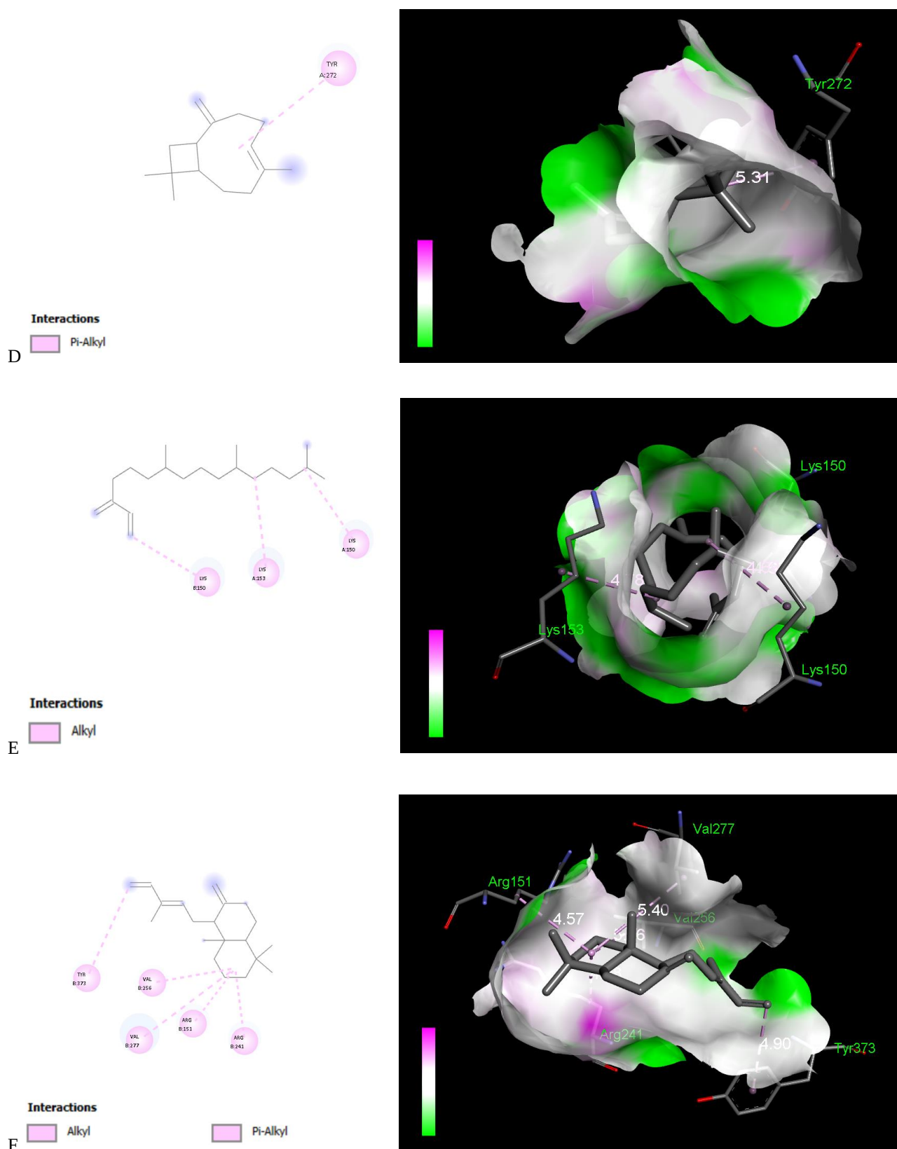
Figure 5. The 2D diagrams and 3D interaction profiles illustrating ligand binding for six compounds within the binding site of PBP2a. A: Interaction distances, A: Eucalyptol, B: Thujone, C: Camphor, D: Caryophyllene, E: Neophytadiene, F: Naphthalene.
