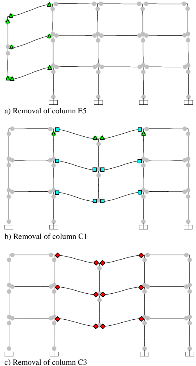
Figure 9. Fiber hinge damage results in the government building. *Gray-filled circle: no damage, green-filled triangle: limited damage, cyan-filled square: moderate damage, pink-filled star: severe damage (collapse prevention), red-filled diamond: failure (collapse).
