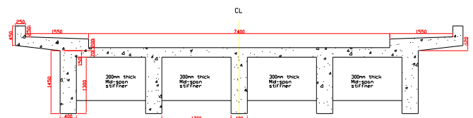
Figure 1. The elevation, the underside view and cross-section of Metsimothlabe Bridge
